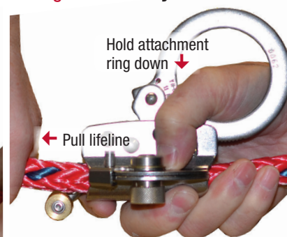
Fig.16b Mobility test
