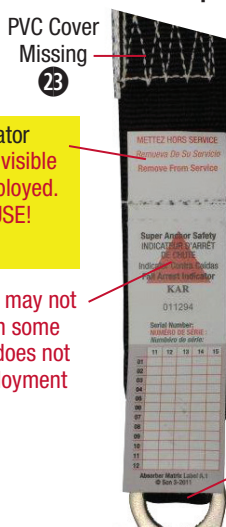
Fig.11 Energy absorber has been deployed.
