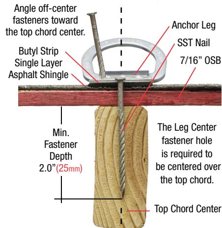
Anchor/Fastener Attachment Over Asphalt Shingles
