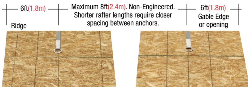
Anchor Spacing
