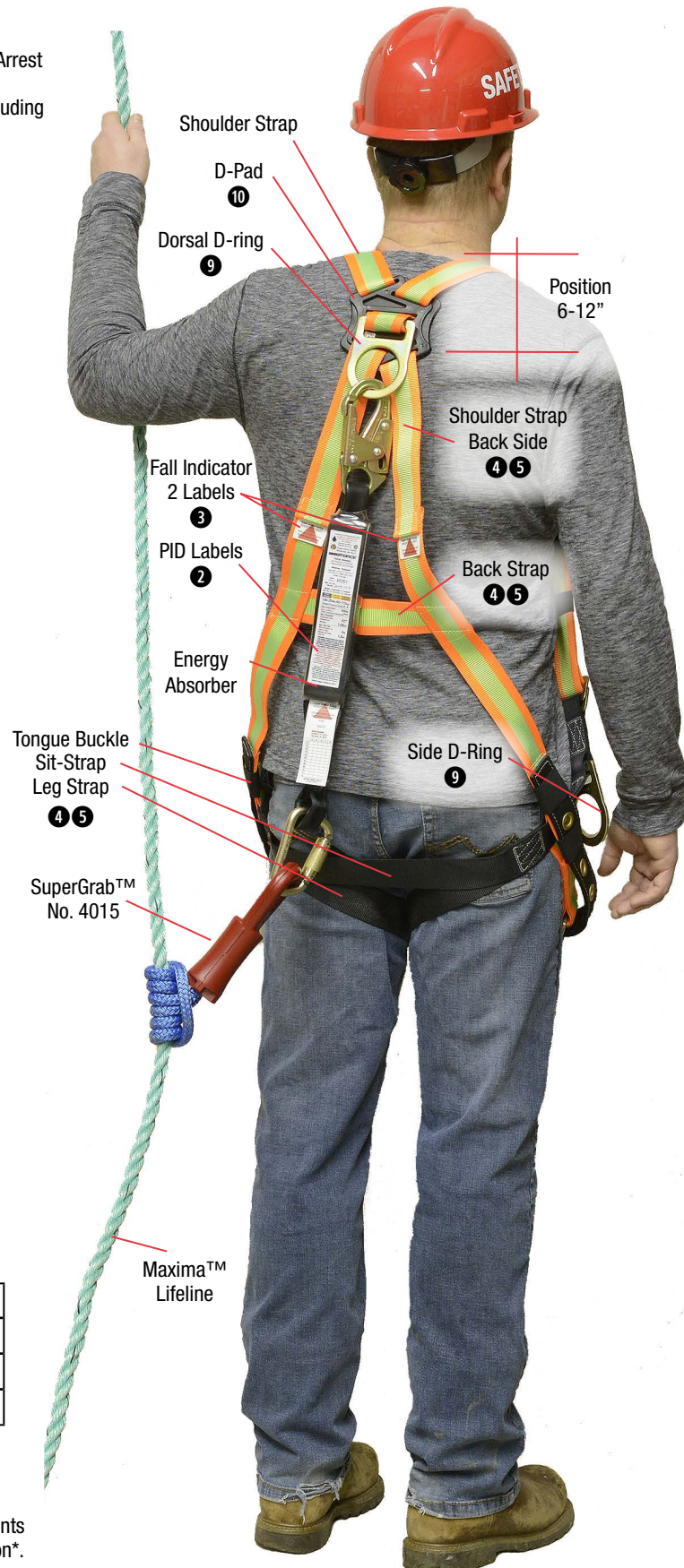
Fig.1 TB-6067 3-D Harness
