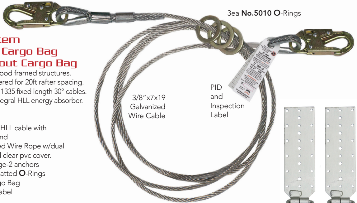
No.3013-D Hinge-2
