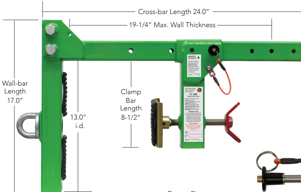
Detent Pin w/shock cord tether.
