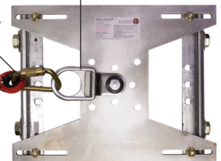
"B" end No.1028 Swivel-D
