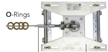
Factory or Field Swage
