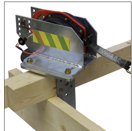
No.1215-UH SRL Holder Complete Kit
