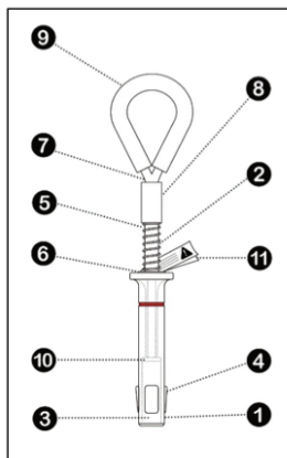
Figure 1: Key components of removable concrete anchor
