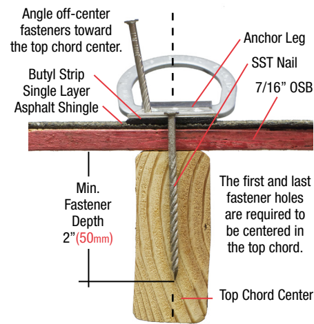
Anchor/Fastener Attachment
